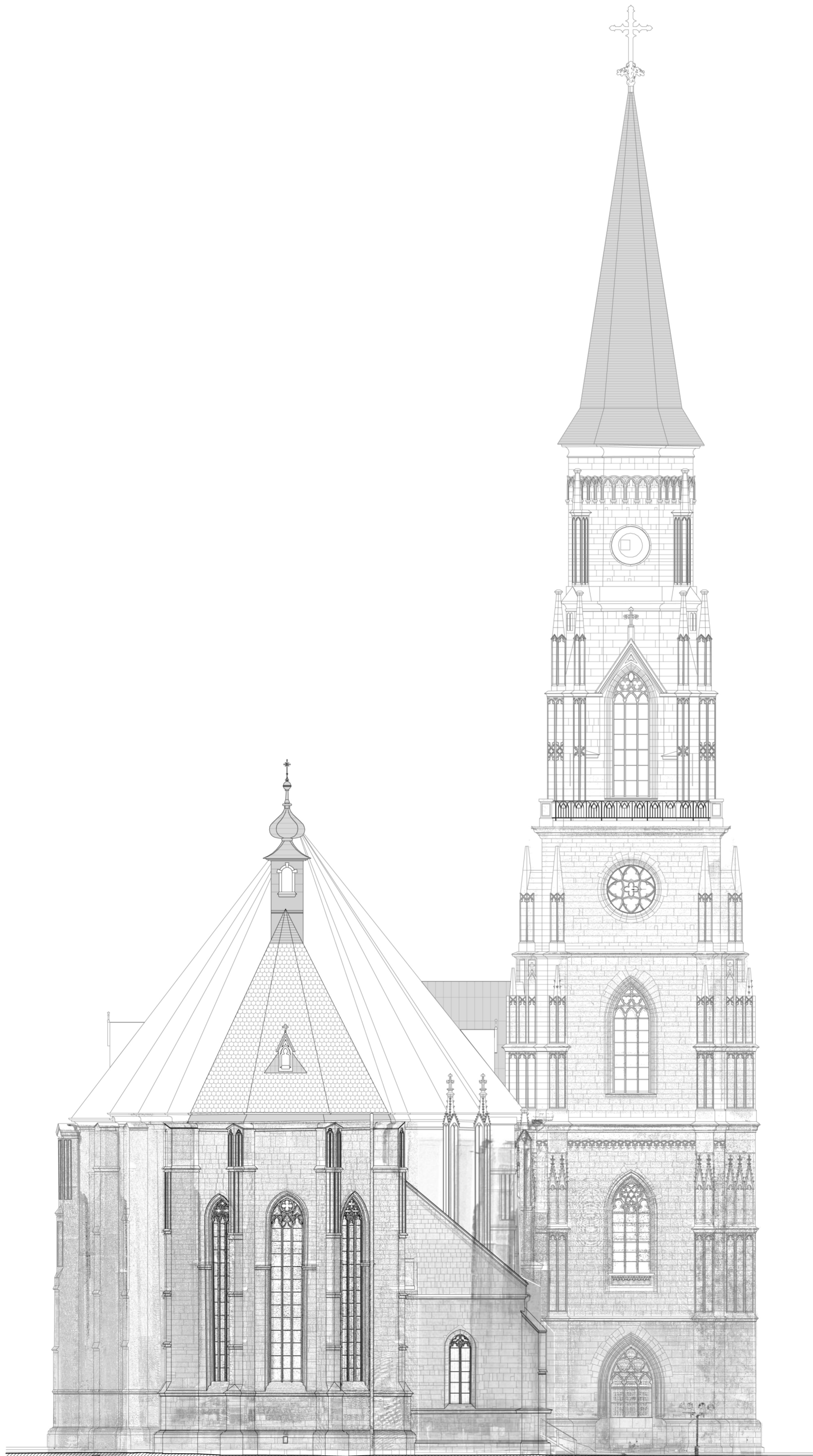
EASTERN FACADE
