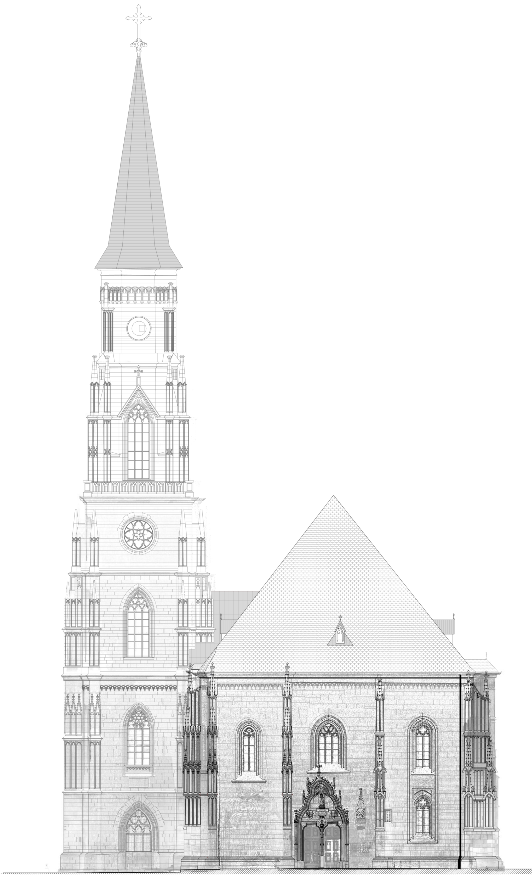
WESTERN FACADE
